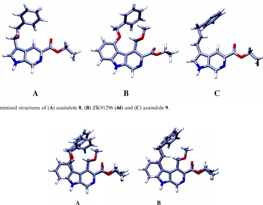
Figure 2. (A) Superposition of ZK91296 ( 4d ) and azaindole 8 . (B) Superposition of ZK91296 ( 4d ) and azaindole 9 .
